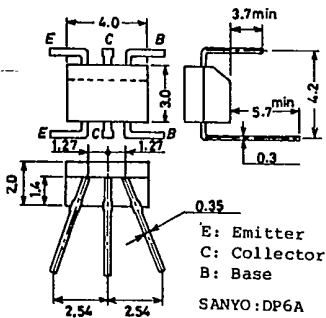
Case Outline 2029A (unit:mm)
