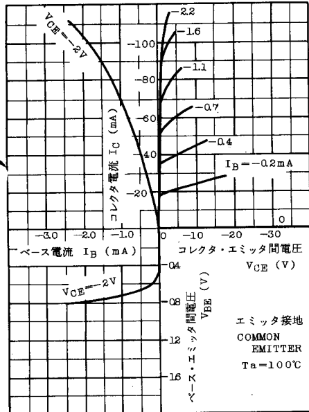
STATIC CHARACTERISTICS
