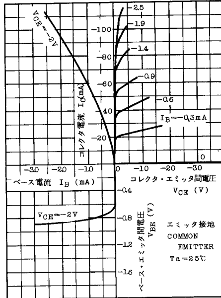
STATIC CHARACTERISTICS
